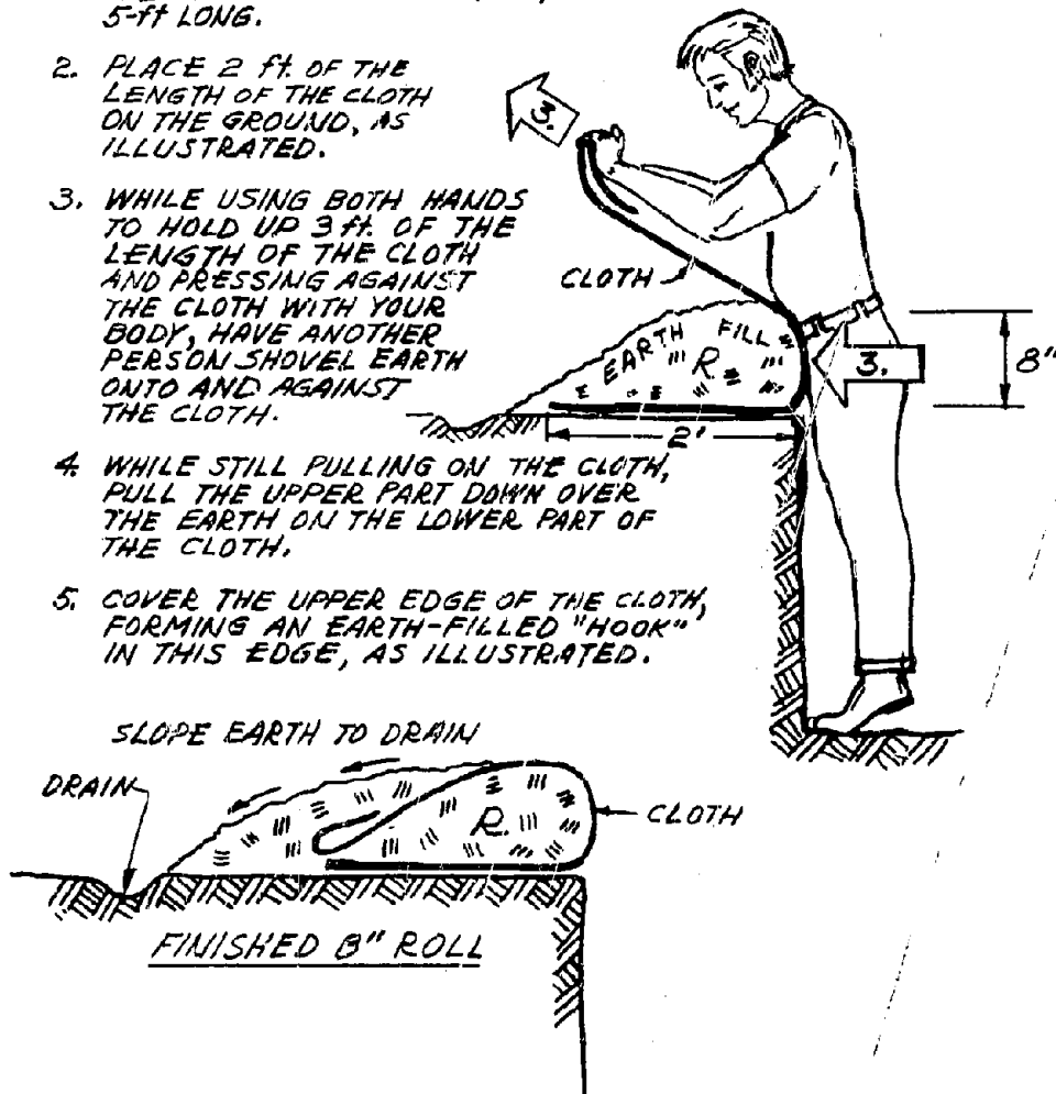
Fig. A-14.2. Door-Over-Trench Shelter, Making a "Roll."
